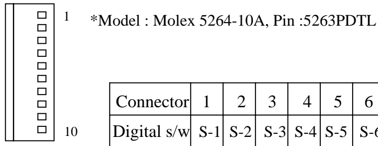
<Connector CN8>
